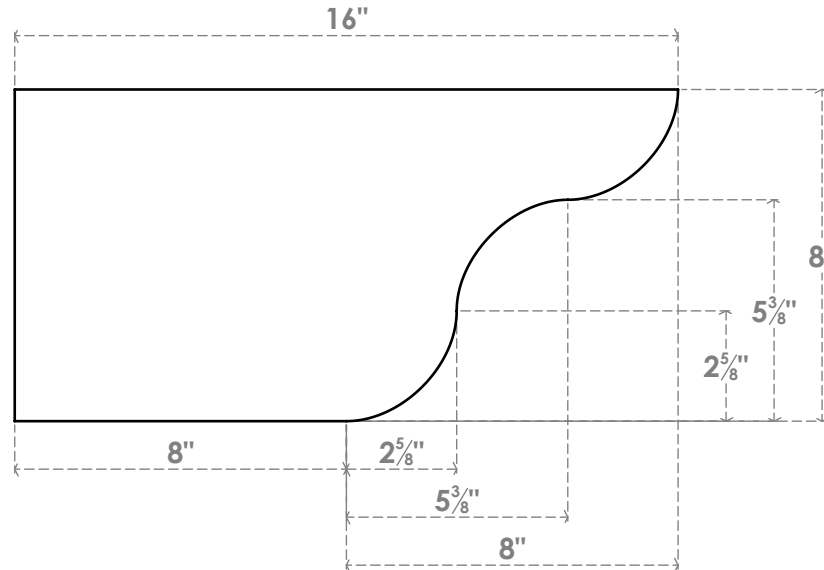
SIDE PROFILE
